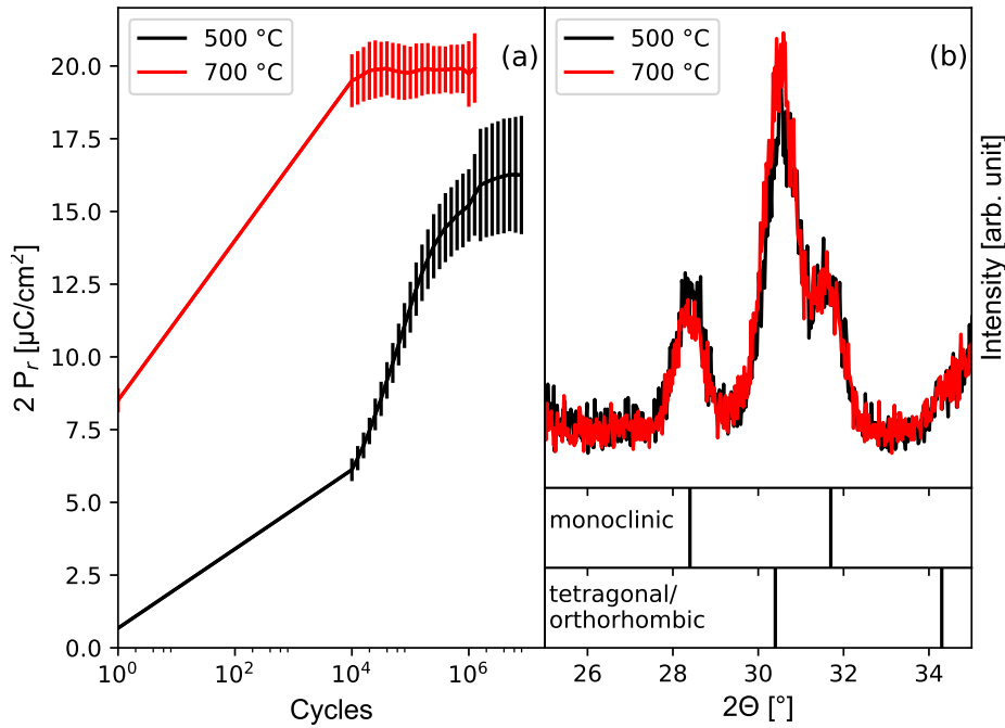
Figure 4.19: Fatigue (a) and GIXRD (b) measurements of a TiN/HfLuO (30 nm)/TiN/Pt sample annealed at 500 °C and 700 °C.
