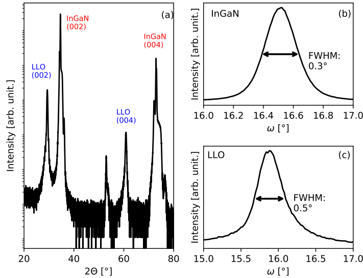
Figure 3.43: (a) \omega - 2\theta scan of the LLO layer on the InGa N substrate in the out-of plane direction revealing the LLO and GaN (002) and (004) reflection. Rocking curve measurement of the InGa N substrate with an FWHM of 0.3° (b) and of the LLO oxide with an FWHM of 0.5° (c).
