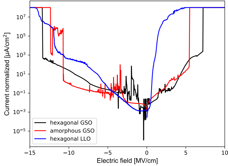
Figure 3.15: IV measurement of hexagonal GSO (black), amorphous GSO (red) and hexagonal LLO (blue) measured up to breakthrough at positive and negative electric field.
