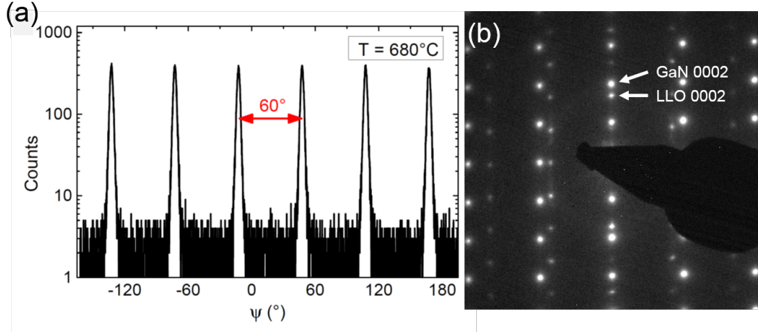
Figure 3.7: (a) \Psi -scan of GSO on GaN of the 1\bar{1}01 reflection showing a sixfold symmetry to prove the hexagonal structure. (b) Diffraction pattern along the (1210) zone axis of LLO on GaN displaying the epitaxial, hexagonal growth by the LLO diffraction spots next to the GaN ones. [4]
