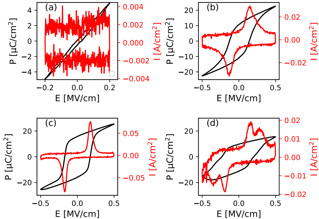
Figure 4.21: Polarisation and current characteristics of an TiN/HfYO/TiN/Pt sample annealed for 30 s in Ar at 600 °C at the initial state (a & b) and after cycling (c). Polarisation and current characteristics of a similar sample annealed at 800 °C for 30 s in Ar (d).
