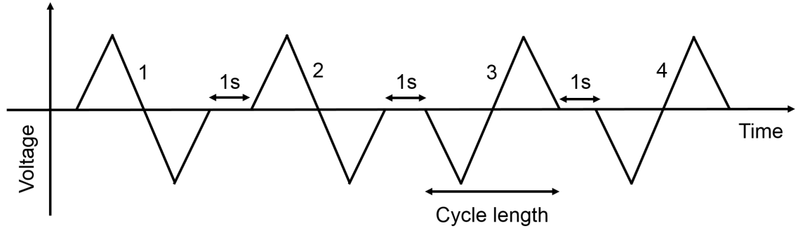
Figure 2.2: Triangular excitation signal for hysteresis measurement. [11]
